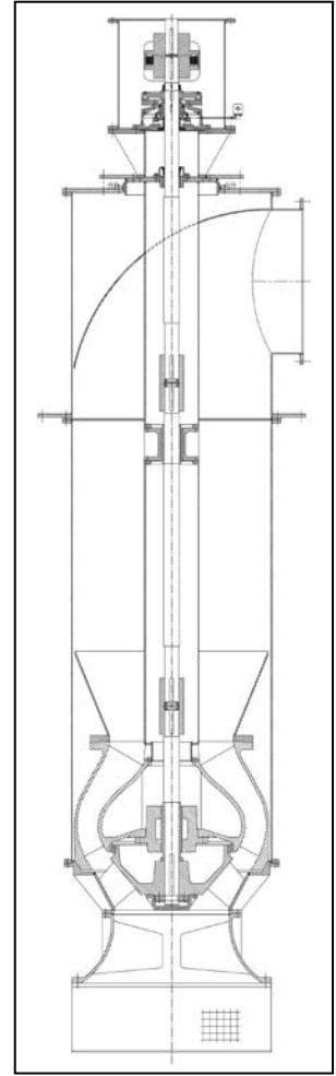
Pull-Out Arrangement
