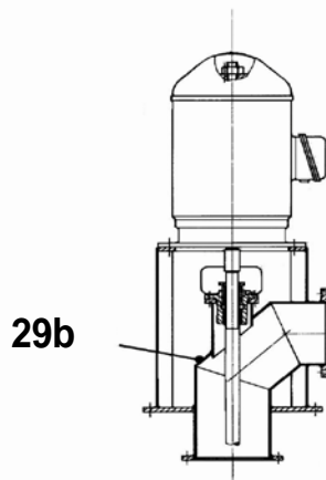
FABRICATED TYPE "B"
