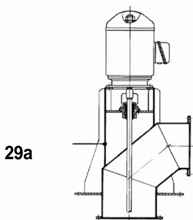
FABRICATED TYPE "A" (ABE)
