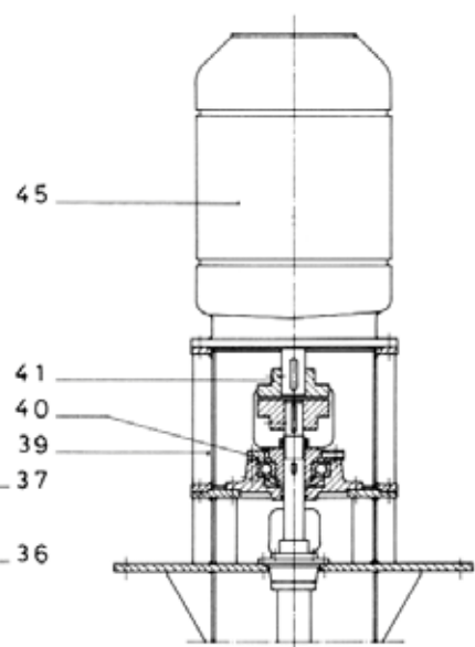
Solid shaft motor. Flexible coupling. Separate axial Thrust bearing
