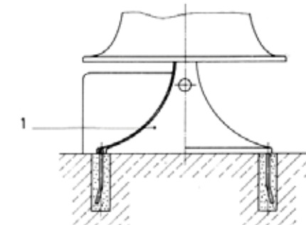
Entry cone to approve suction approach.
